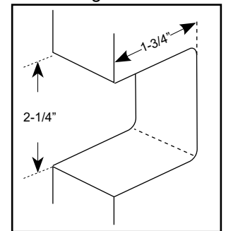
Notching Dimensions
